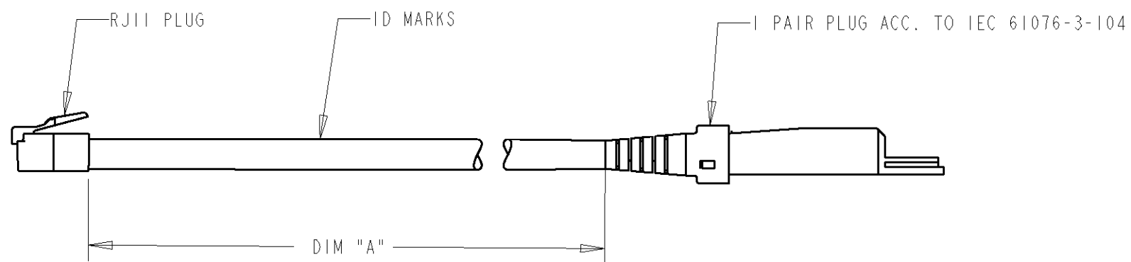
SCHEMATIC VIEW
