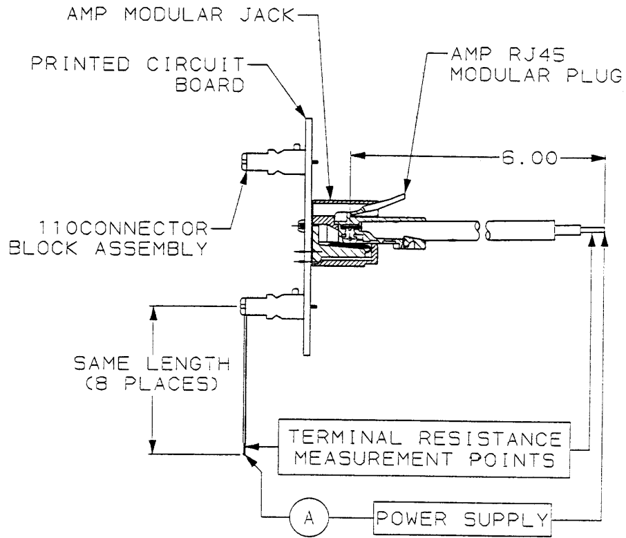
Figure 3 Termination Resistance Measurement Points
