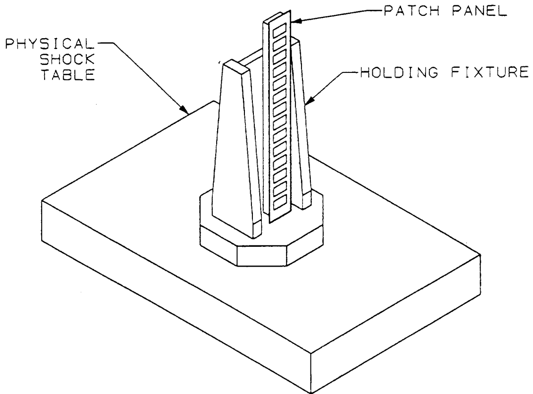
Figure 5 Vibration & Physical Shock Mounting Fixtures
