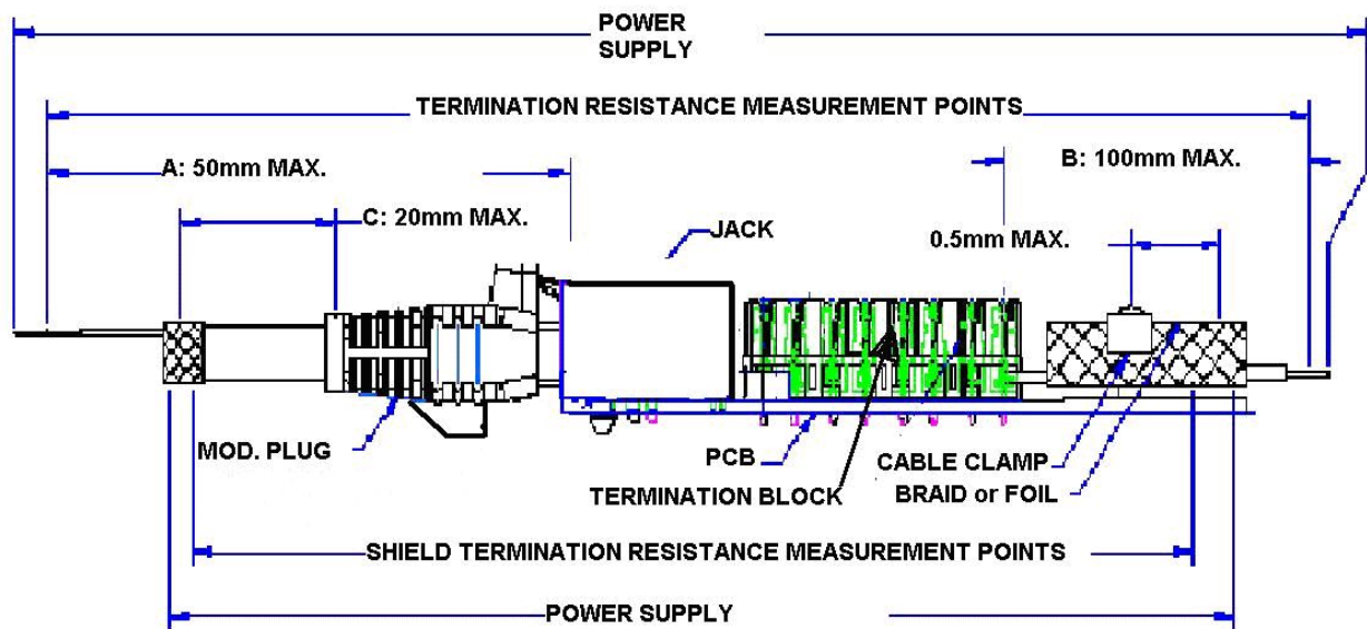
Figure 3 Cat.5E System
