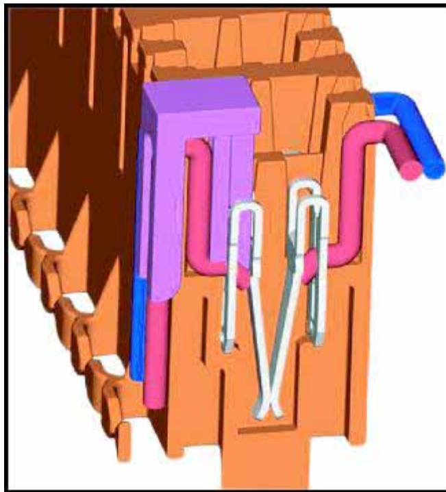
Detail of wire insertion. The excess of wire is cut by a blade incorporated in the terminal design.
